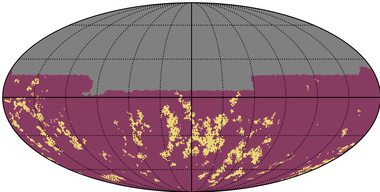
weather_cloudso16v3.4_10yrs u band: Gaps_7hr
