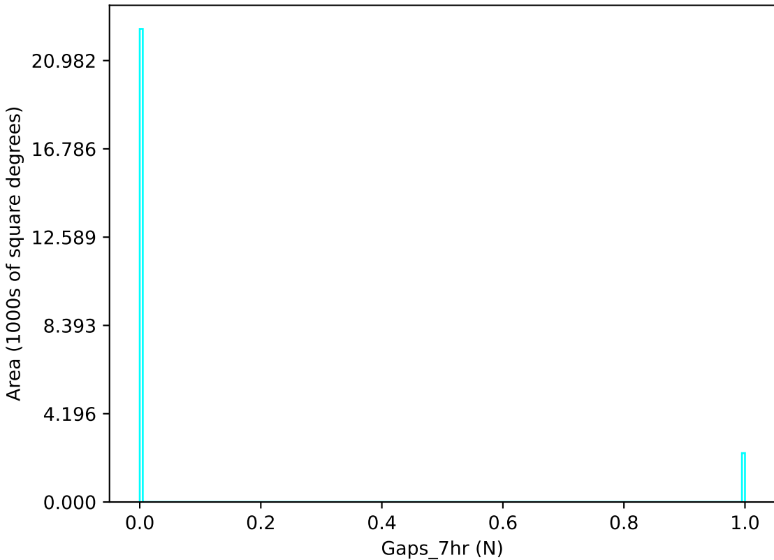
weather_cloudso16v3.4_10yrs u band: Gaps_7hr
