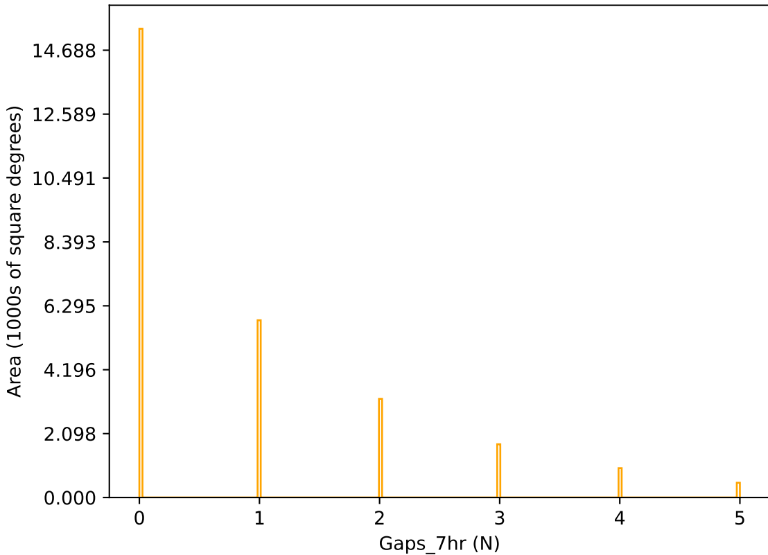
weather_cloudso16v3.4_10yrs r band: Gaps_7hr
