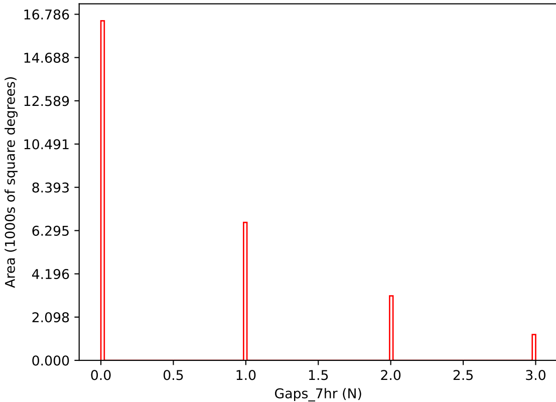
weather_cloudso16v3.4_10yrs i band: Gaps_7hr
