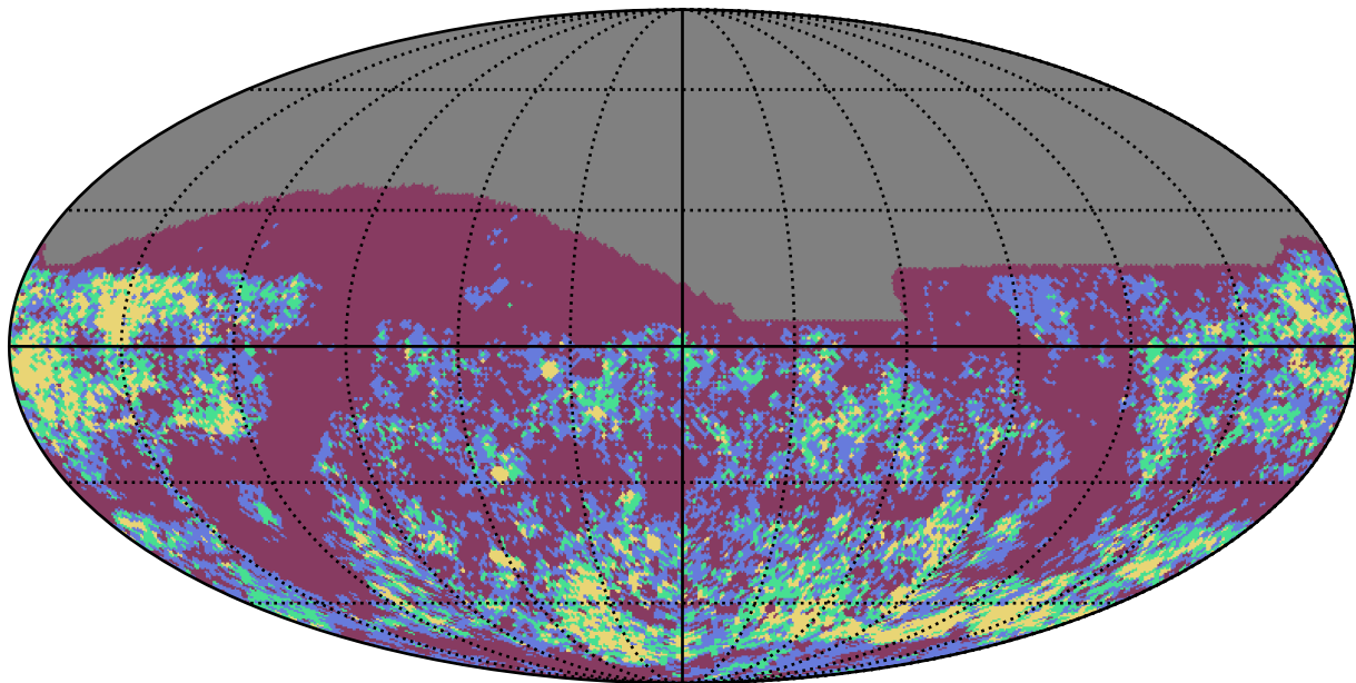
weather_cloudso16v3.4_10yrs z band: Gaps_3hr
