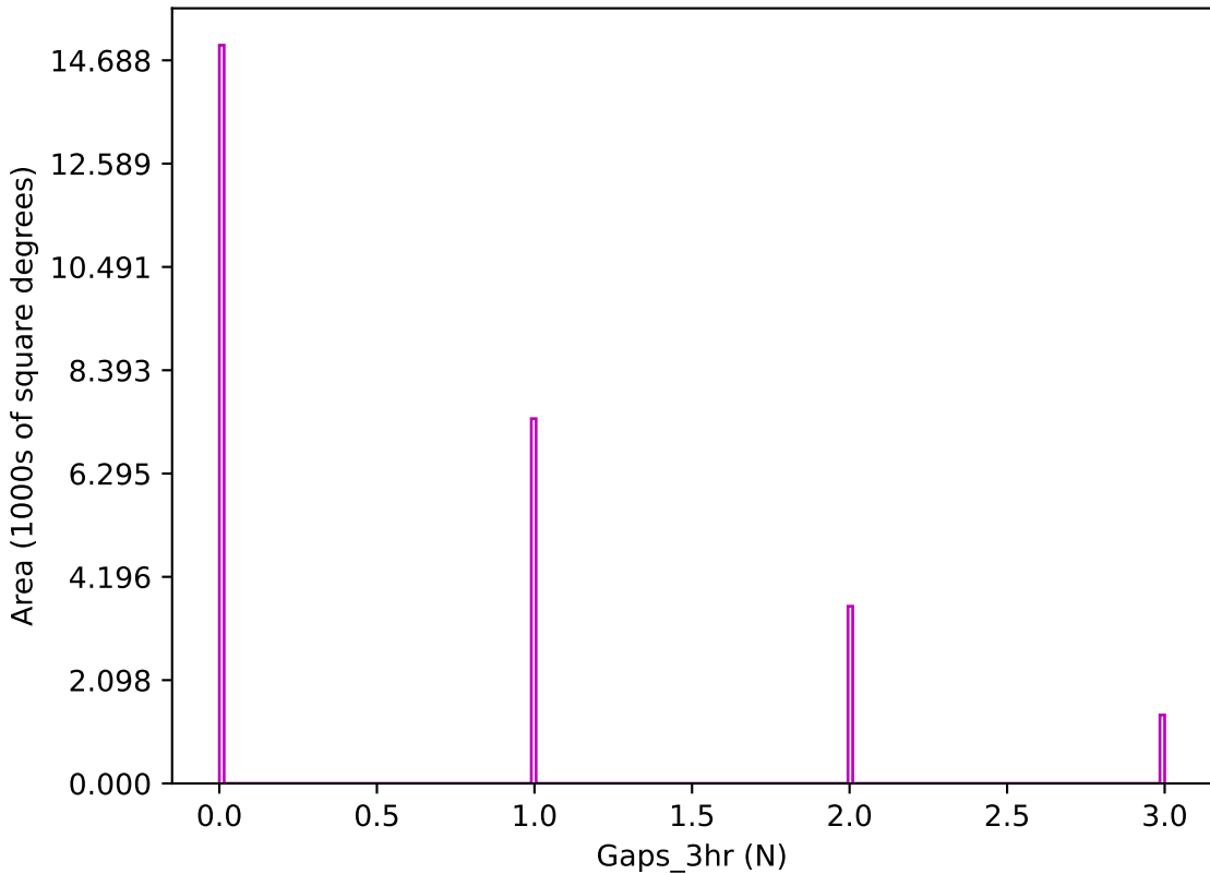
weather_cloudso16v3.4_10yrs z band: Gaps_3hr
