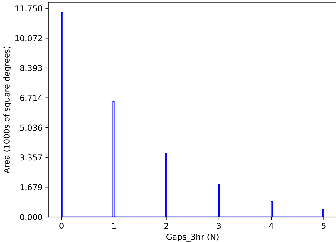
weather_cloudso16v3.4_10yrs y band: Gaps_3hr
