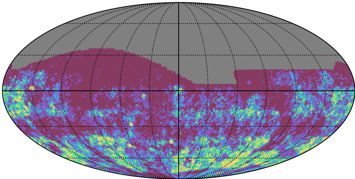
weather_cloudso16v3.4_10yrs r band: Gaps_3hr
