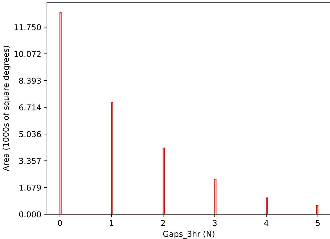
weather_cloudso16v3.4_10yrs i band: Gaps_3hr
