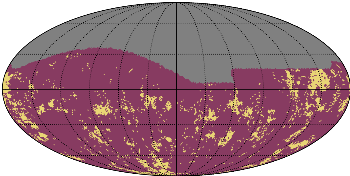
weather_cloudso16v3.4_10yrs g band: Gaps_3hr
