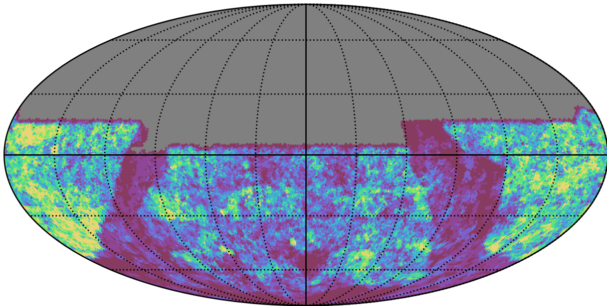
weather_cloudso16v3.4_10yrs u band: Gaps_24hr
