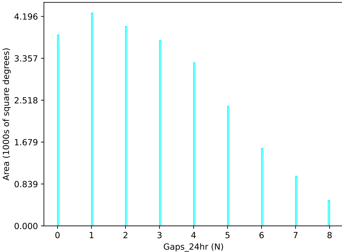
weather_cloudso16v3.4_10yrs u band: Gaps_24hr
