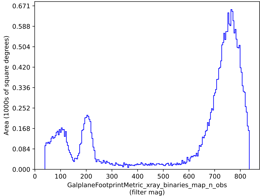
weather_cloudso16v3.4_10yrs : GalplaneFootprintMetric_xray_binaries_map_n_obs
