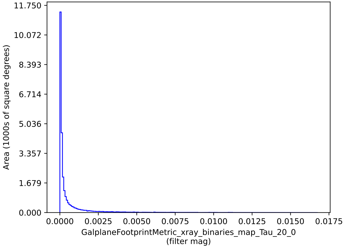
weather_cloudso16v3.4_10yrs : GalplaneFootprintMetric_xray_binaries_map_Tau_20_0
