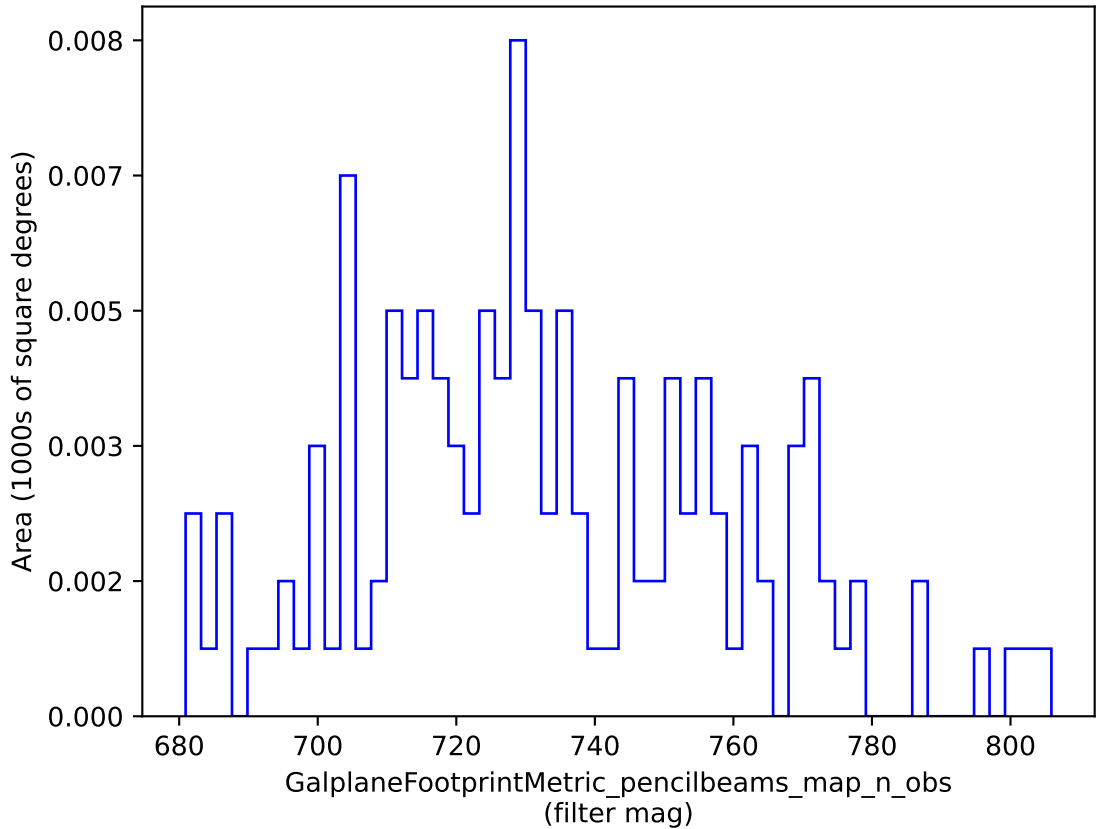
weather_cloudso16v3.4_10yrs : GalplaneFootprintMetric_pencilbeams_map_n_obs
