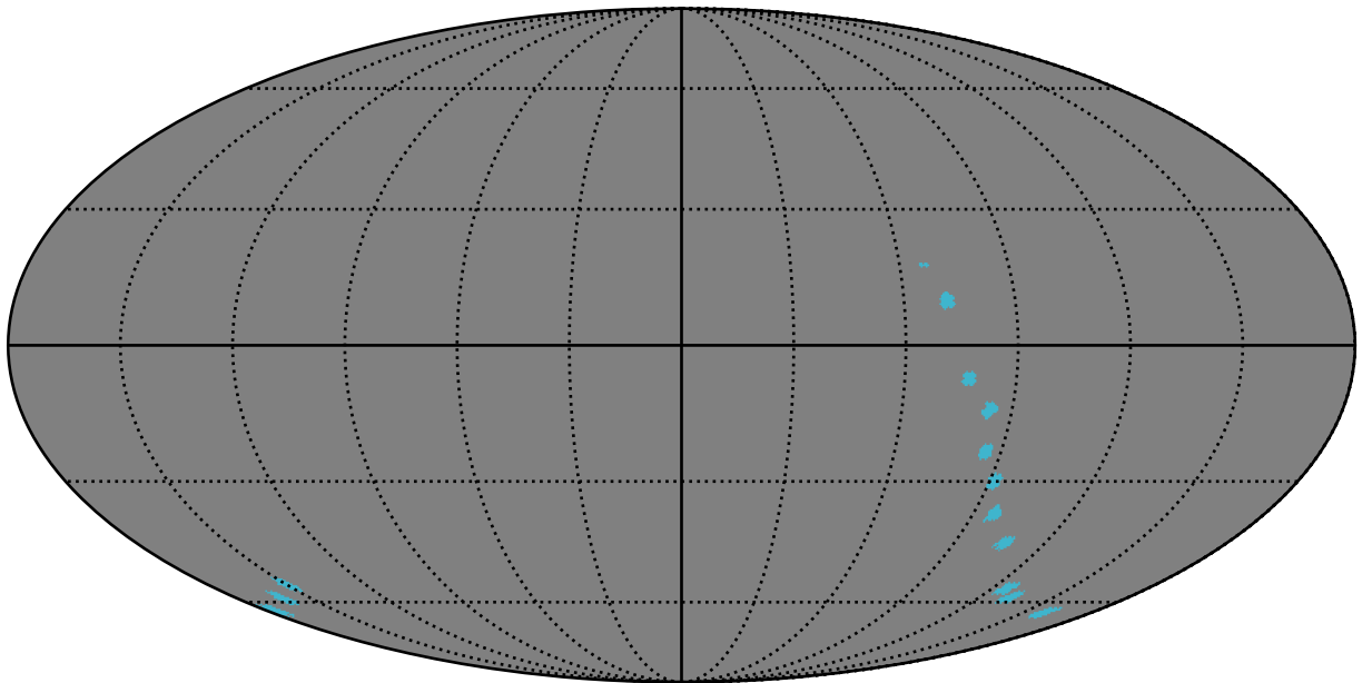
weather_cloudso16v3.4_10yrs : GalplaneFootprintMetric_pencilbeams_map_Tau_2_0
