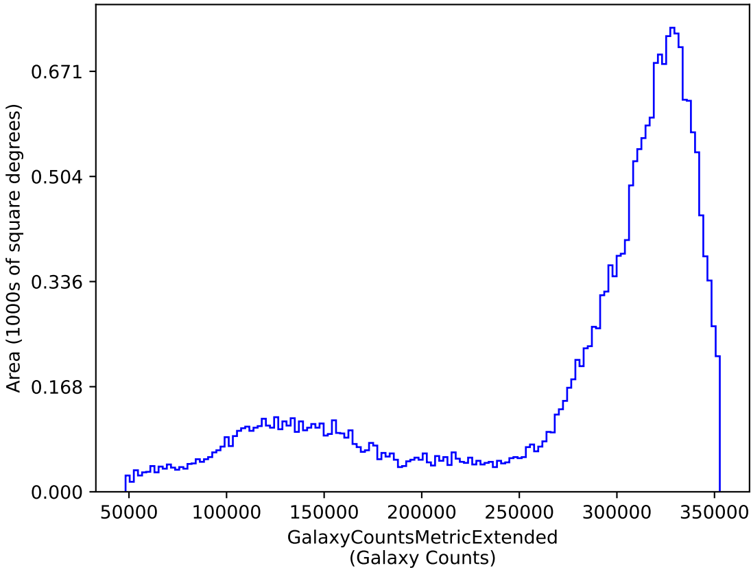
weather_cloudso16v3.4_10yrs y: GalaxyCountsMetricExtended
