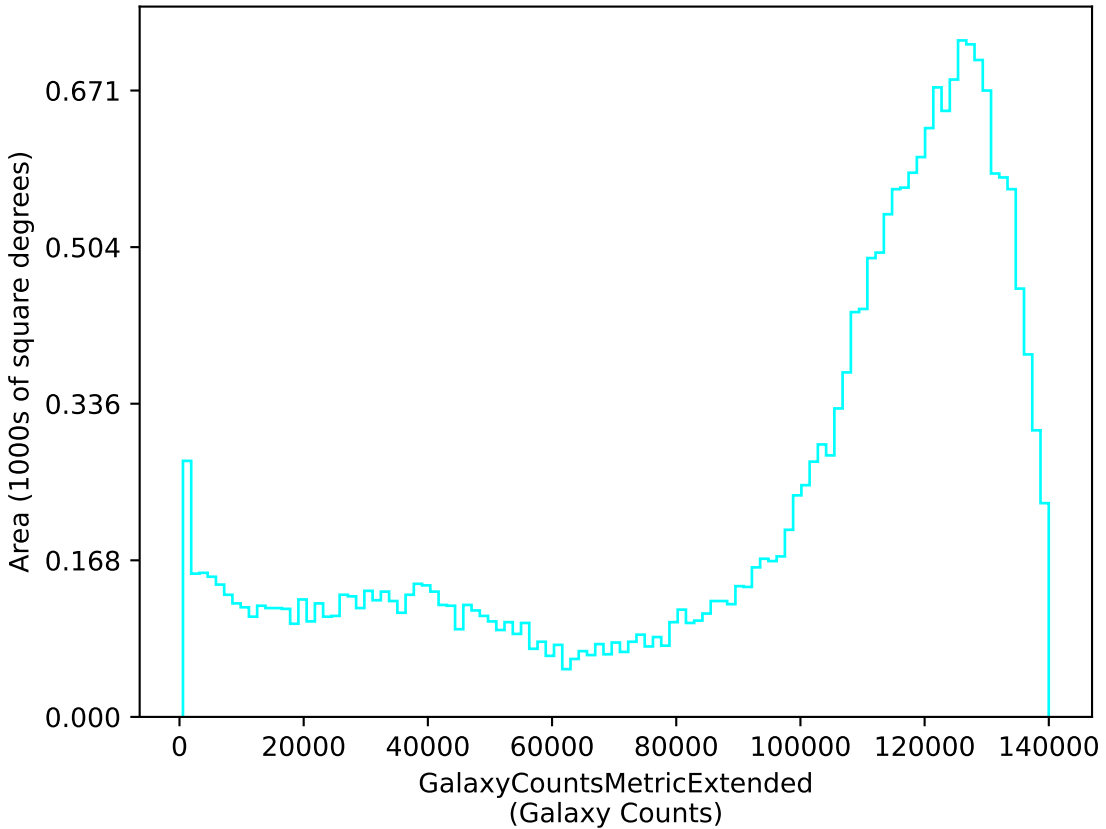
weather_cloudso16v3.4_10yrs u: GalaxyCountsMetricExtended
