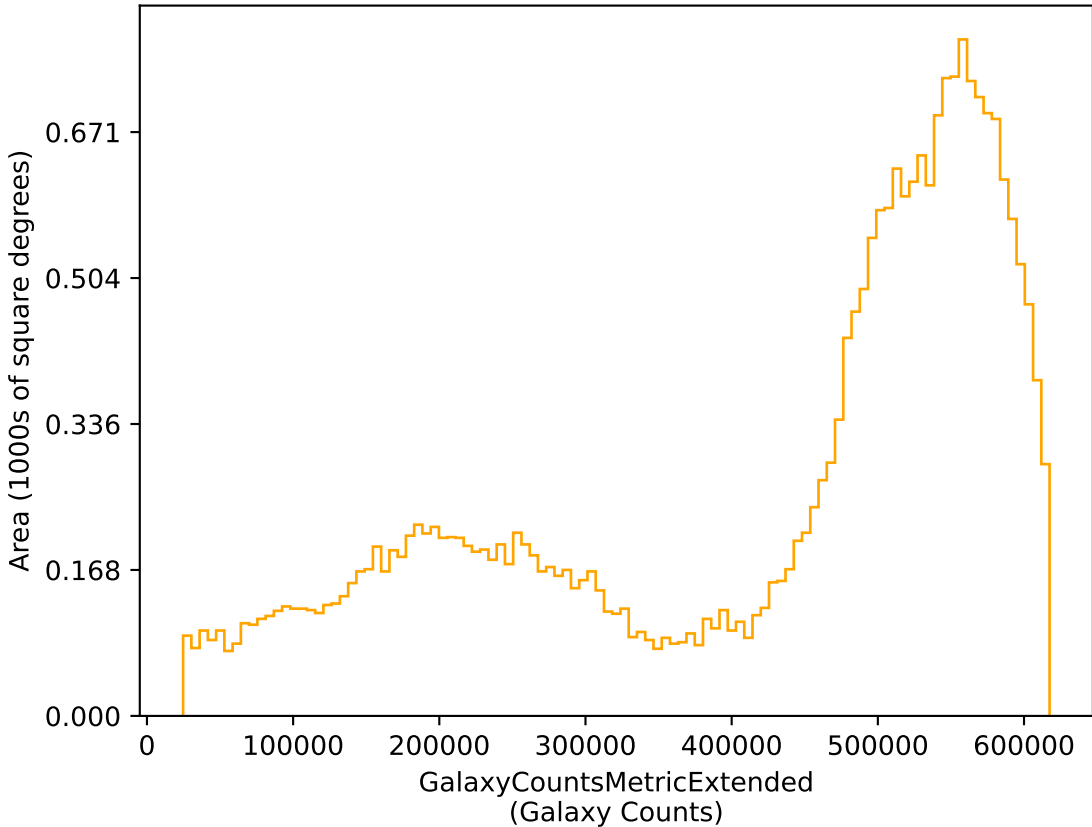
weather_cloudso16v3.4_10yrs r: GalaxyCountsMetricExtended
