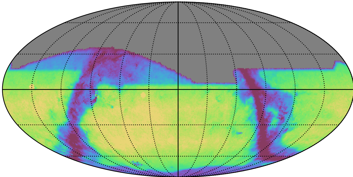
weather_cloudso16v3.4_10yrs i: GalaxyCountsMetricExtended
