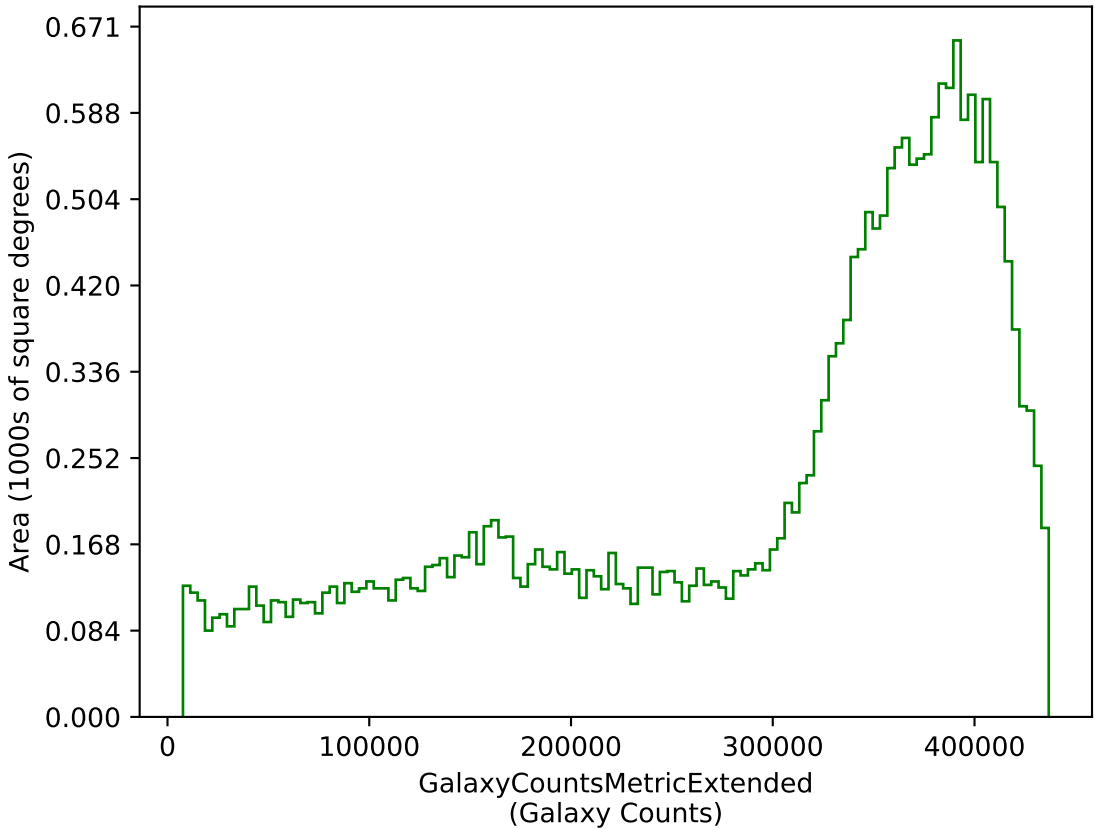
weather_cloudso16v3.4_10yrs g: GalaxyCountsMetricExtended
