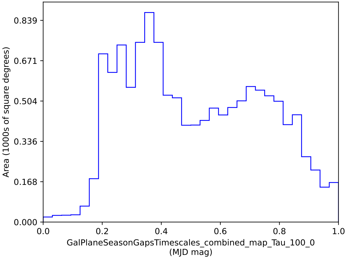
weather_cloudso16v3.4_10yrs : GalPlaneSeasonGapsTimescales_combined_map_Tau_100_0
