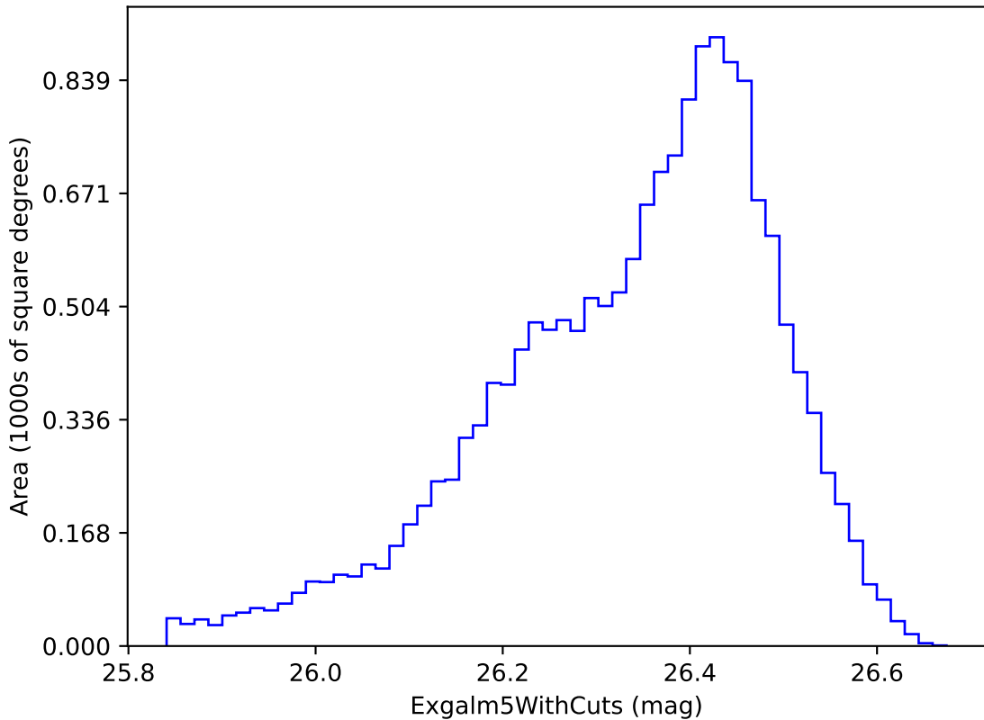
weather_cloudso16v3.4_10yrs i band non-DD year 9: Exgal5WithCuts
