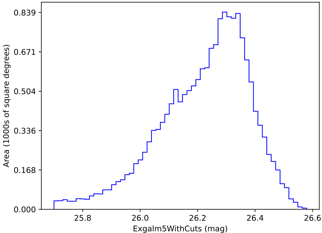
weather_cloudso16v3.4_10yrs i band non-DD year 7: ExgalM5WithCuts
