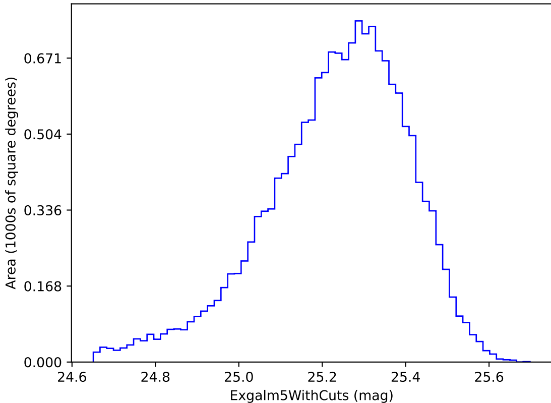
weather_cloudso16v3.4_10yrs i band non-DD year 1: ExgalM5WithCuts
