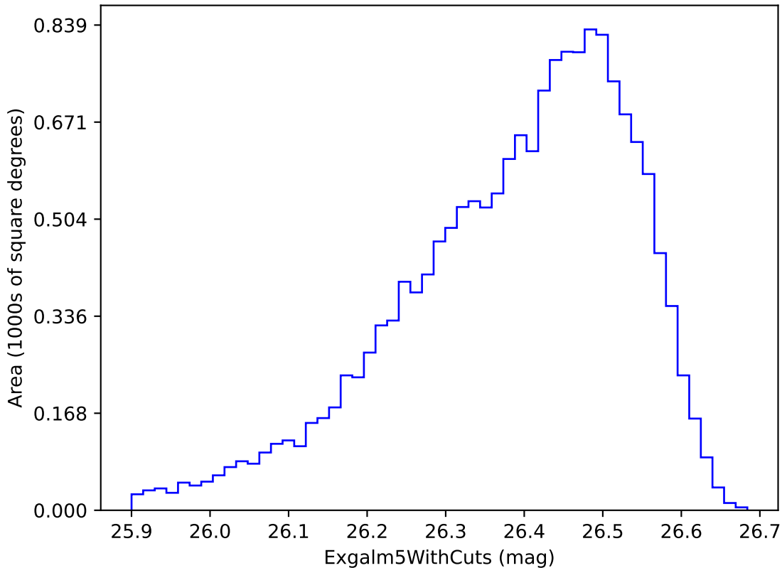
weather_cloudso16v3.4_10yrs i band non-DD year 10: Exgalml5WithCuts
