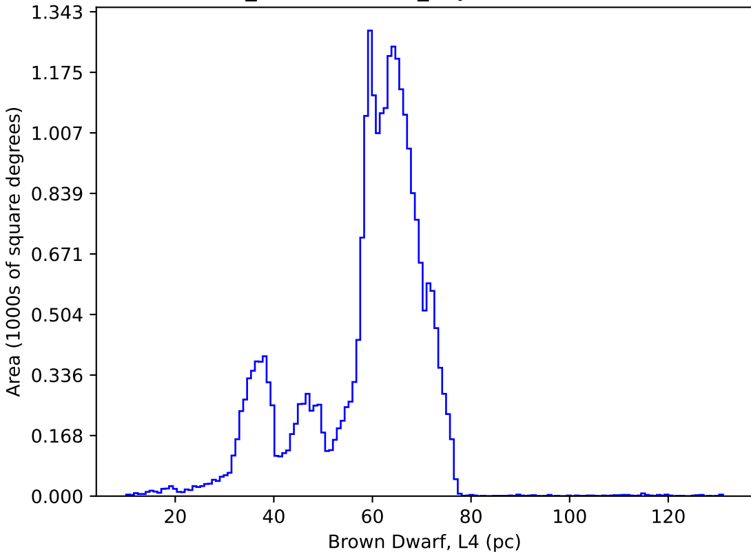
weather_cloudso16v3.4_10yrs : Brown Dwarf, L4
