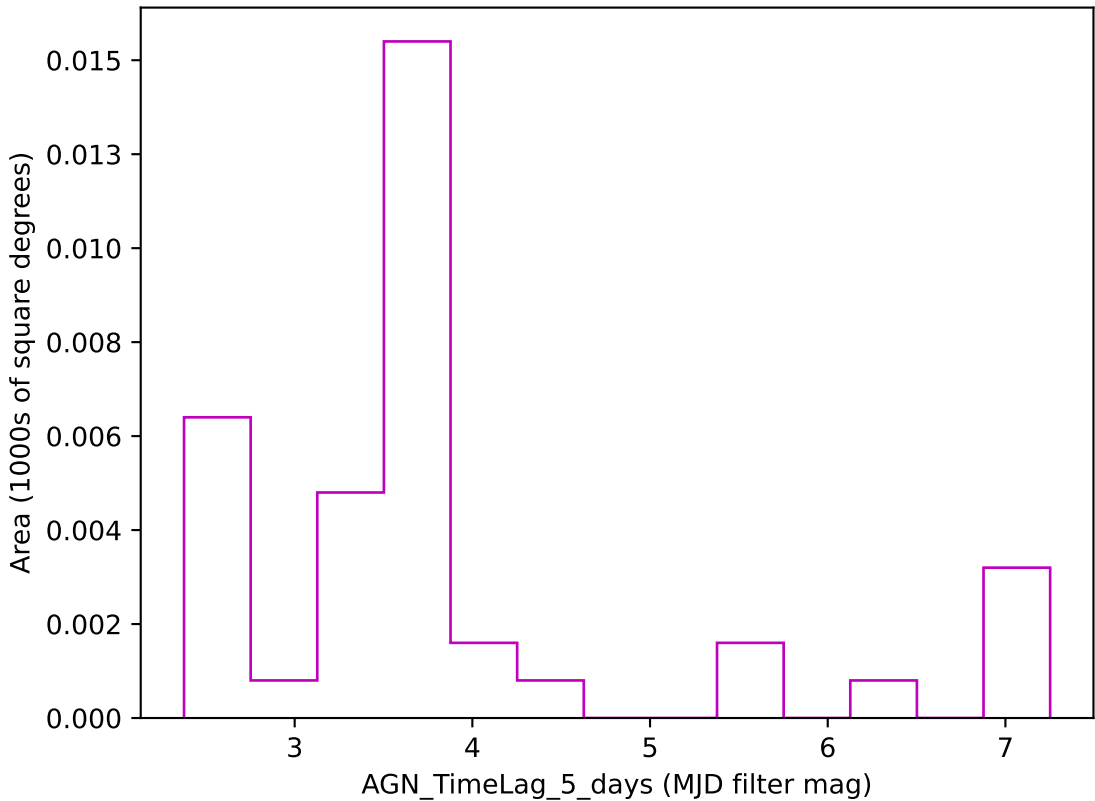
weather_cloudso16v3.4_10yrs z band: AGN_TimeLag_5_days
