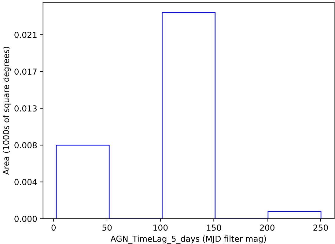
weather_cloudso16v3.4_10yrs y band: AGN_TimeLag_5_days
