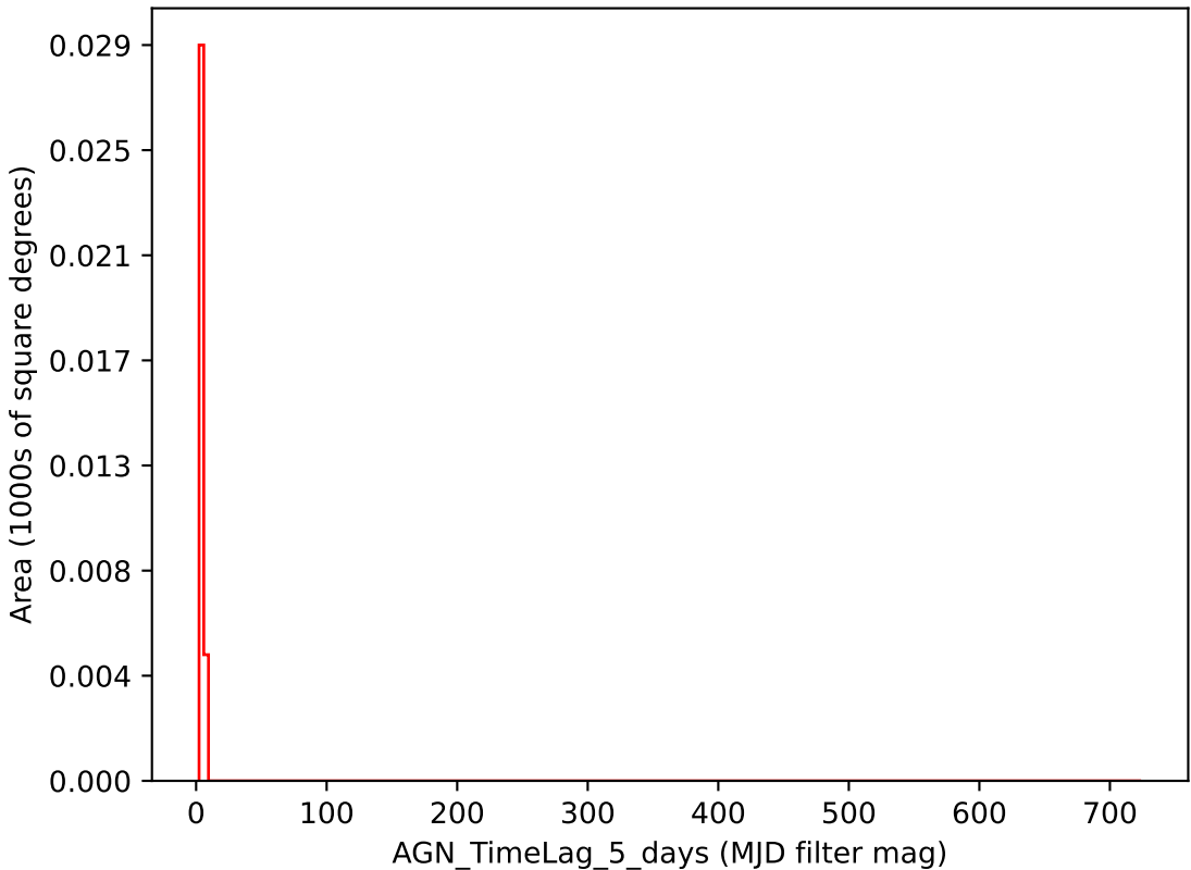
weather_cloudso16v3.4_10yrs i band: AGN_TimeLag_5_days
