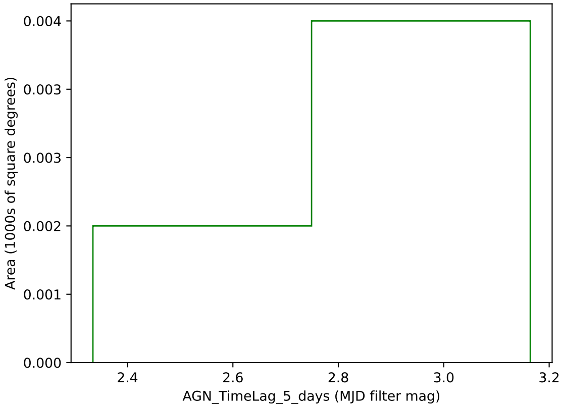
weather_cloudso16v3.4_10yrs g band: AGN_TimeLag_5_days
