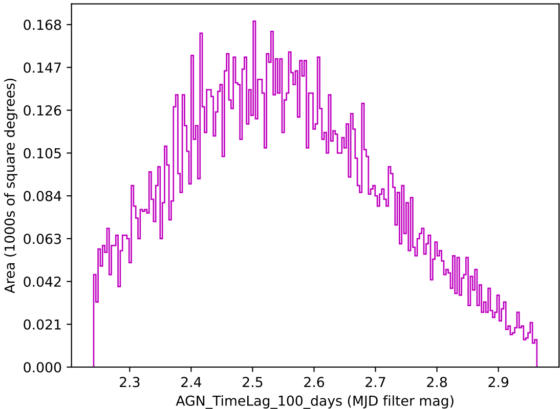
weather_cloudso16v3.4_10yrs z band: AGN_TimeLag_100_days
