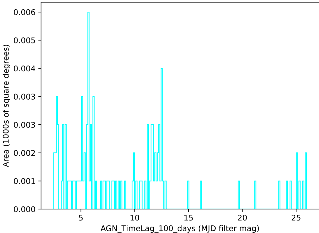
weather_cloudso16v3.4_10yrs u band: AGN_TimeLag_100_days
