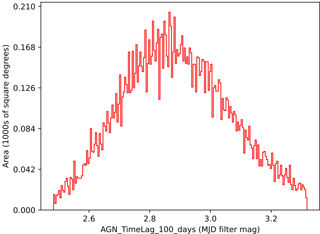
weather_cloudso16v3.4_10yrs i band: AGN_TimeLag_100_days
