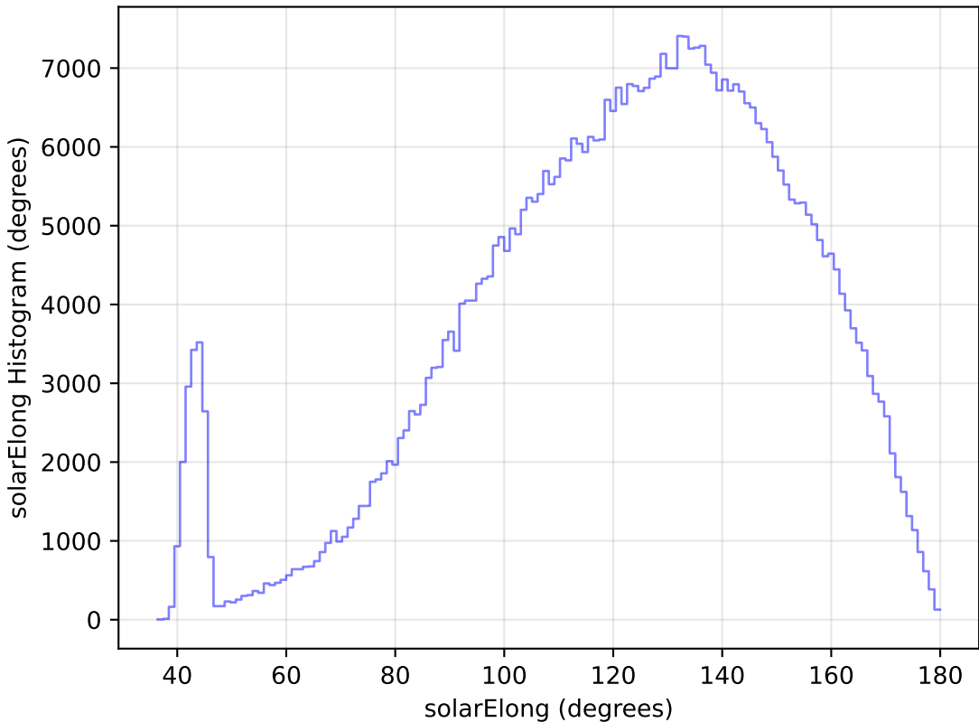
weather_cloudso16v3.4_10yrs WFD r band: solarElong Histogram
