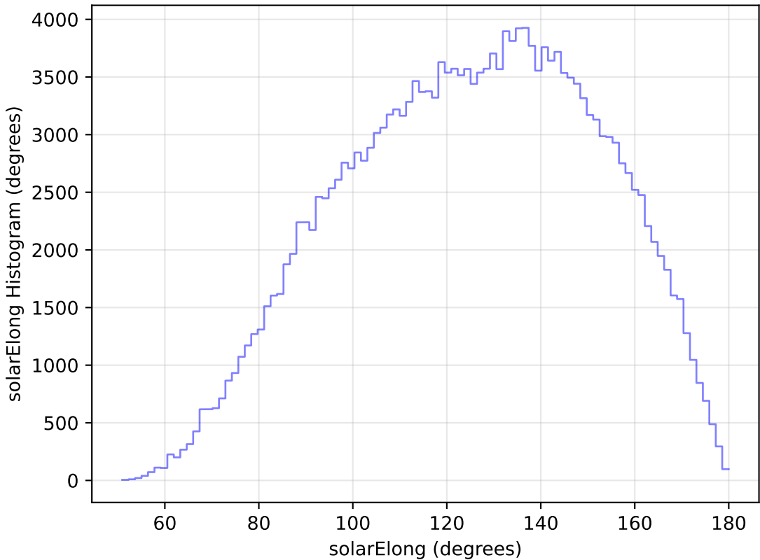
weather_cloudso16v3.4_10yrs WFD g band: solarElong Histogram
