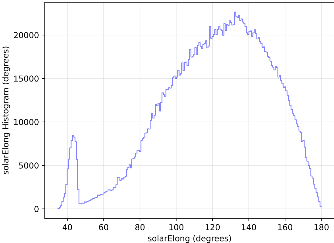
weather_cloudso16v3.4_10yrs WFD all bands: solarElong Histogram
