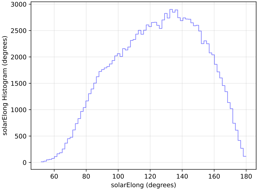
weather_cloudso16v3.4_10yrs All sky u band: solarElong Histogram
