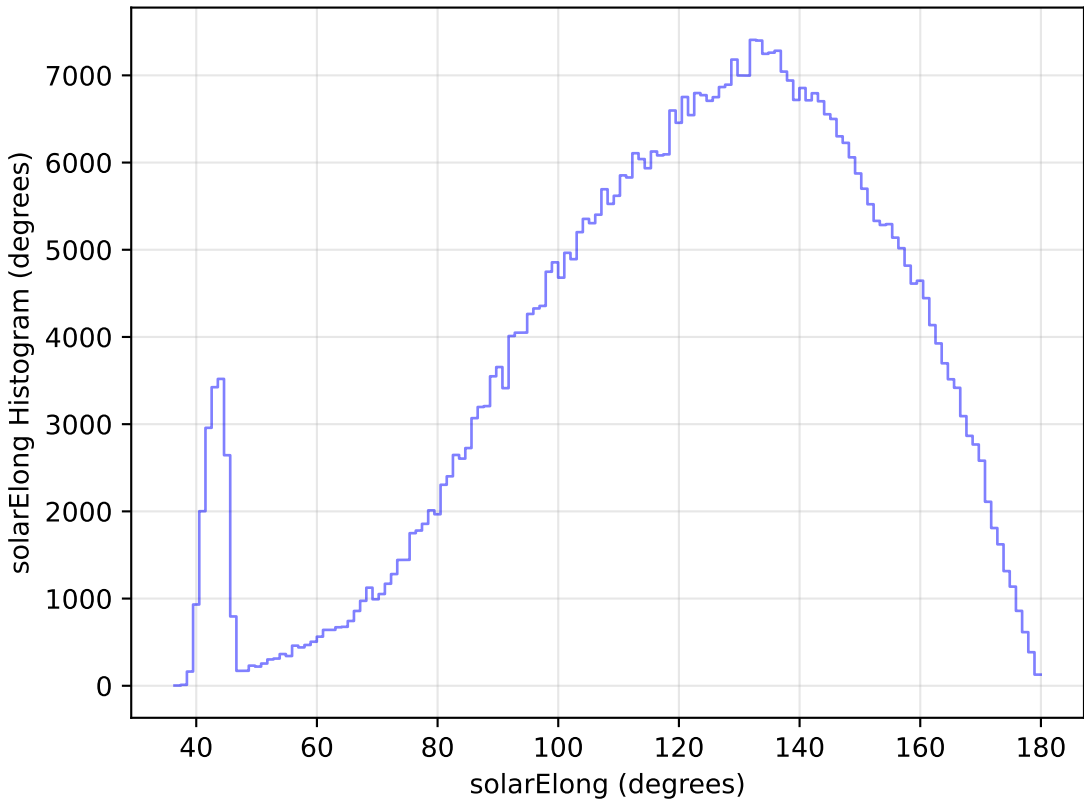
weather_cloudso16v3.4_10yrs All sky r band: solarElong Histogram
