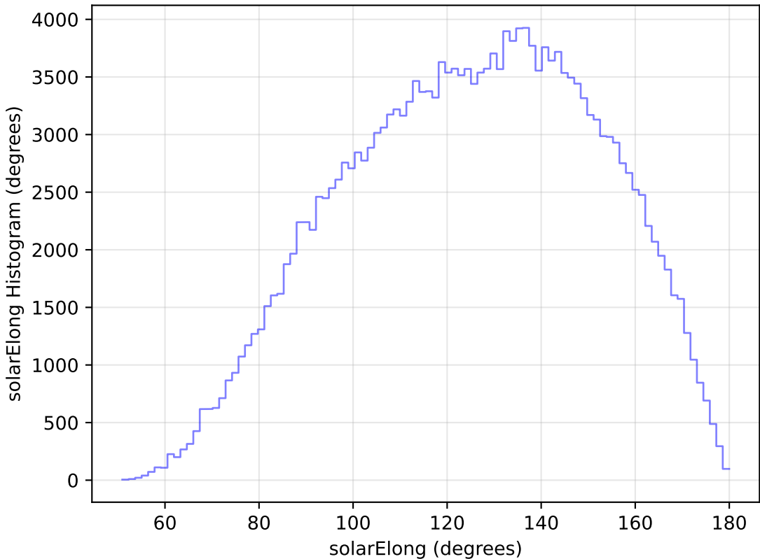
weather_cloudso16v3.4_10yrs All sky g band: solarElong Histogram
