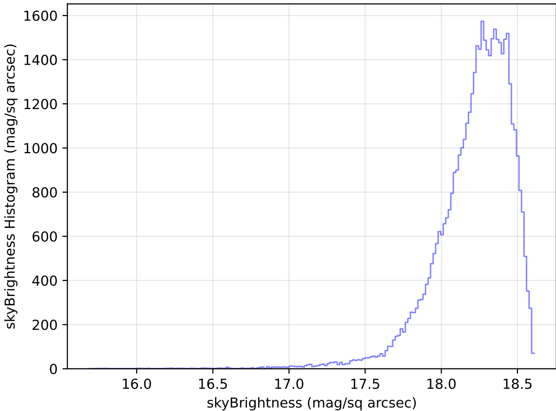
weather_cloudso16v3.4_10yrs Yr 1 y band: skyBrightness Histogram
