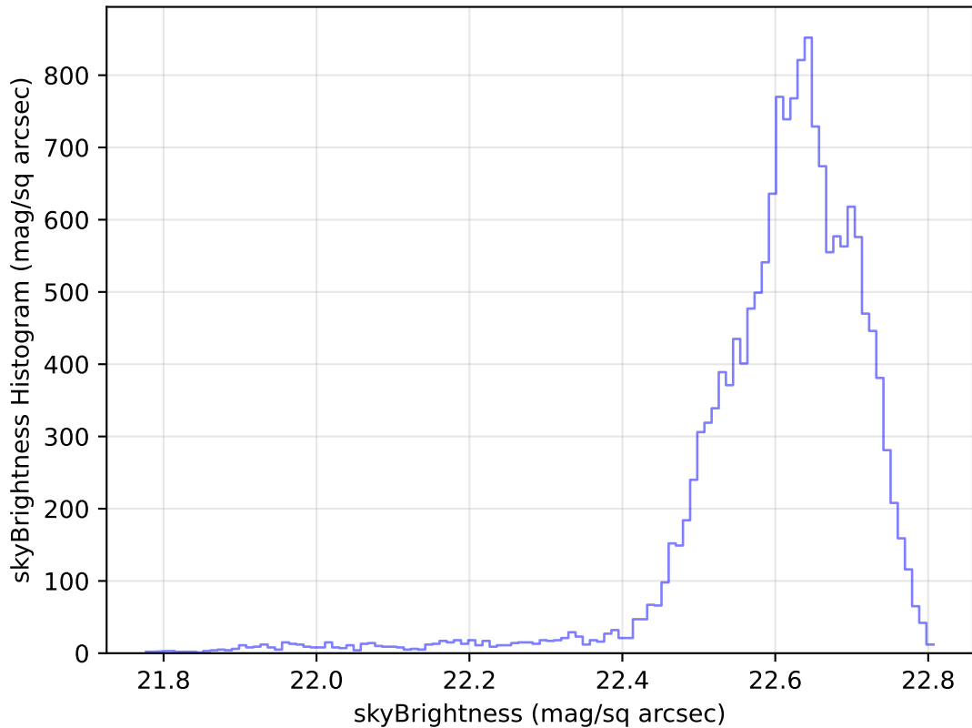
weather_cloudso16v3.4_10yrs Yr 1 u band: skyBrightness Histogram
