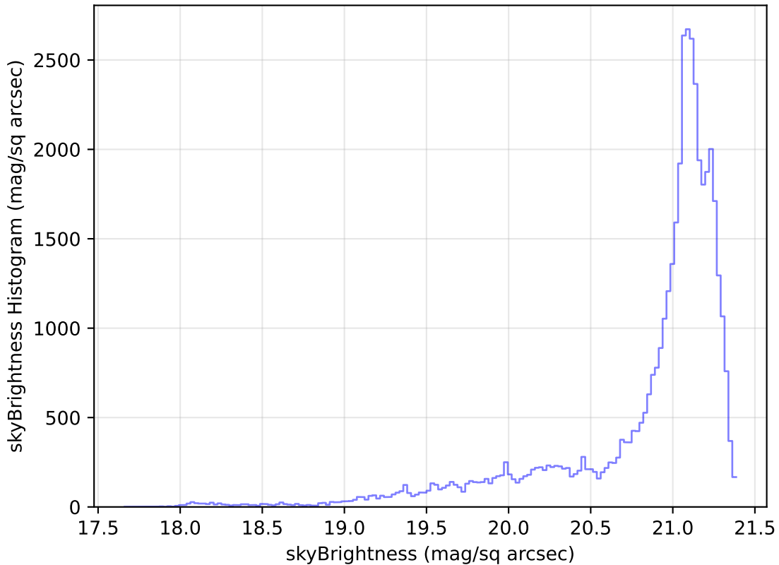
weather_cloudso16v3.4_10yrs Yr 1 r band: skyBrightness Histogram
