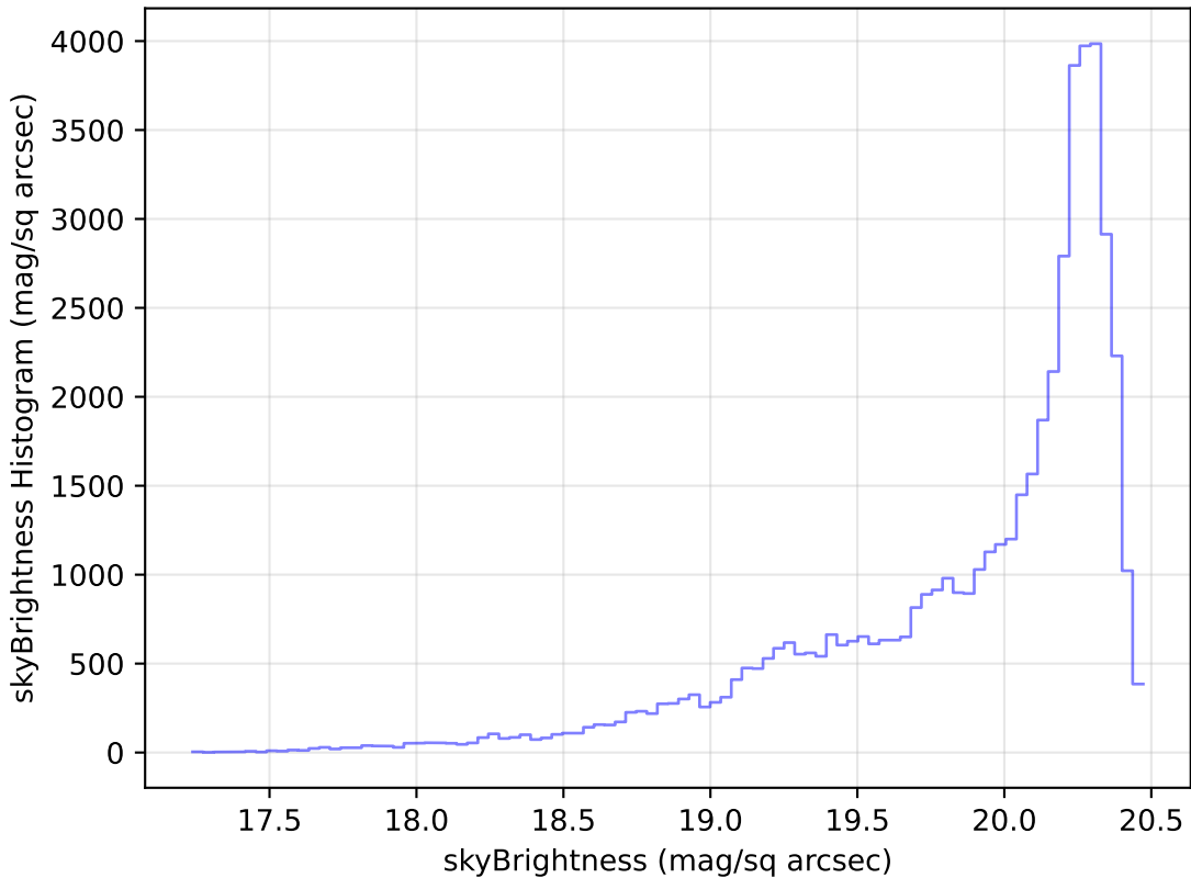
weather_cloudso16v3.4_10yrs Yr 1 i band: skyBrightness Histogram
