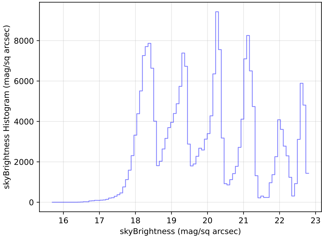
weather_cloudso16v3.4_10yrs Yr 1 all bands: skyBrightness Histogram
