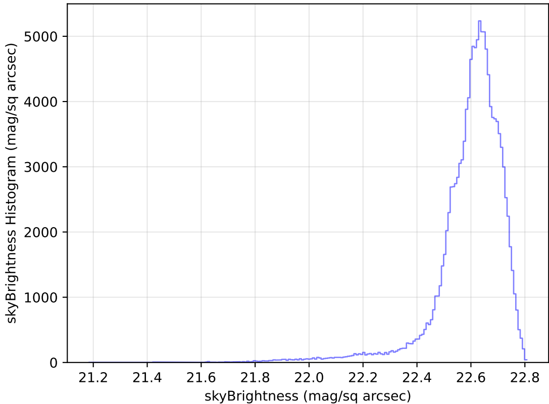
weather_cloudso16v3.4_10yrs WFD u band: skyBrightness Histogram
