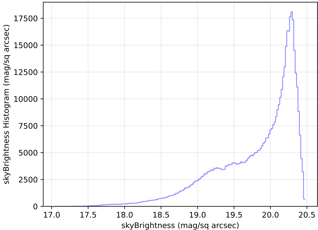
weather_cloudso16v3.4_10yrs WFD i band: skyBrightness Histogram
