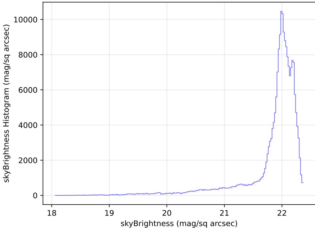
weather_cloudso16v3.4_10yrs WFD g band: skyBrightness Histogram
