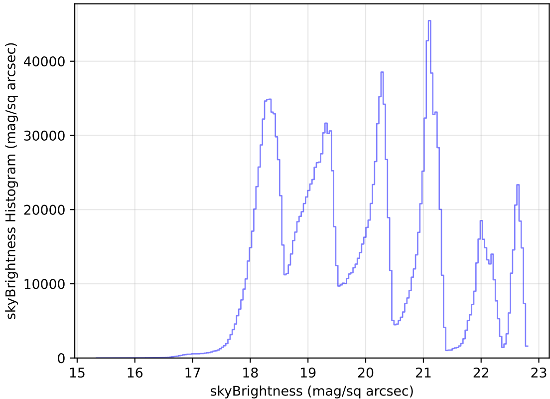
weather_cloudso16v3.4_10yrs WFD all bands: skyBrightness Histogram
