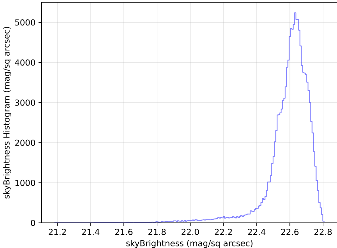
weather_cloudso16v3.4_10yrs All sky u band: skyBrightness Histogram
